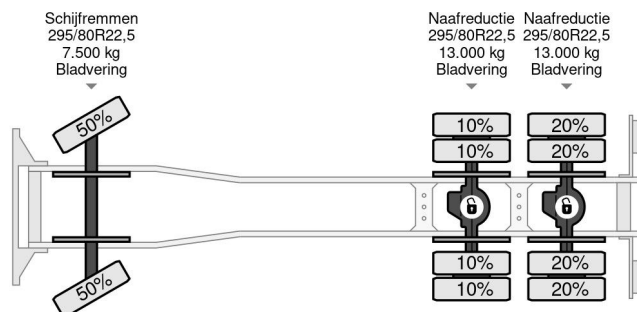
Mercedes-Benz Actros 2643 B 6x4 FULL STEEL CHASSIS (...) Referentienummer: SN 61137496 Z
