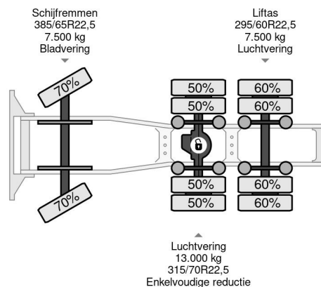
DAF XF 105.460 SUPERSPACECAB 6x2 (EURO 5 / AS-TR...
