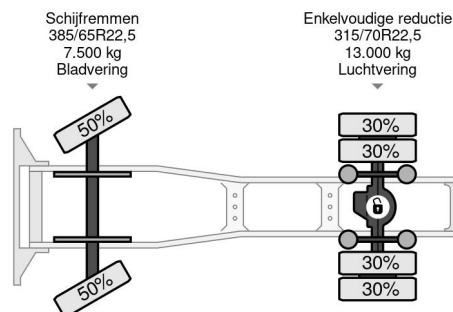
DAF XF 105.460 ATE SPACECAB (EURO 5 / AS-TRONIC GEARBOX / ZF-INTARDER / 870+430 LITER DIESEL TANK / AIRCONDITIONING) 4x2
