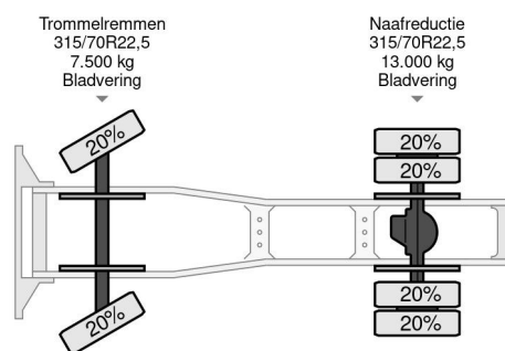
Renault G340 Manager 4x2 TRACTOR (MECHANICAL PUMP...
