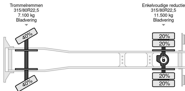
MAN 12.232 F90 (6-CILINDER) FULL STEEL SUSPEN... 4x2
