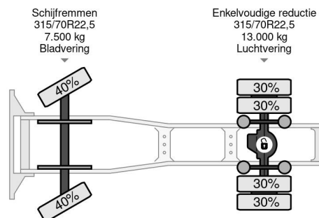
DAF XF 105.460 SPACECAB (ZF MANUAL GEARBOX / ... 4x2
