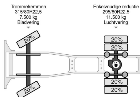
DAF 95.480 XF SPACECAB (EURO 3 / ZF16 MANUAL ... 4x2
