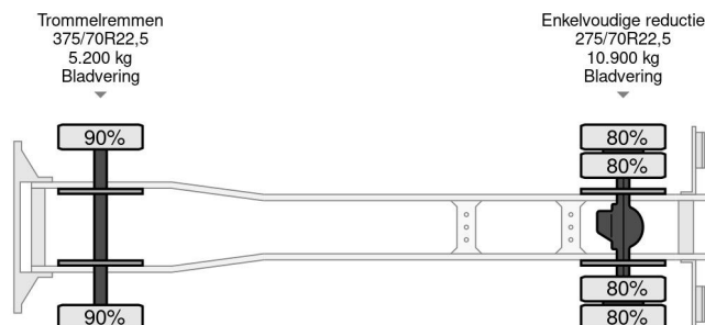
Renault Midliner 180 -15/D RHD WITH RAVO KZ7082/1... 4x2
