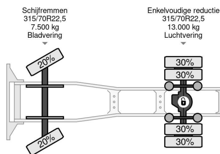
DAF XF 105.460 SPACECAB (ZF-MANUAL GEARBOX /... 4x2
