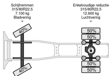
Renault Magnum 440 E-TECH (MACK ENGINE / ZF16 ... 4x2
