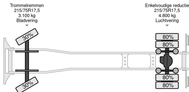
Mercedes-Benz LK 814 (6-CILINDER) WITH OPEN (TE... 4x2
