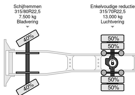
DAF XF 105.460 ATE SPACECAB (EURO 5 / ZF MANU... 4x2
