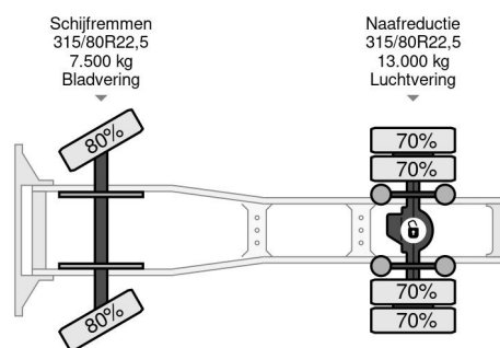
Mercedes-Benz Actros 1843 LS SLEEPERCAB (MP1) ... 4x2
